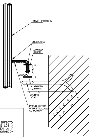
DETALLE 5 BISAGRA PORTON
